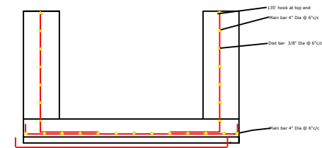
X section
