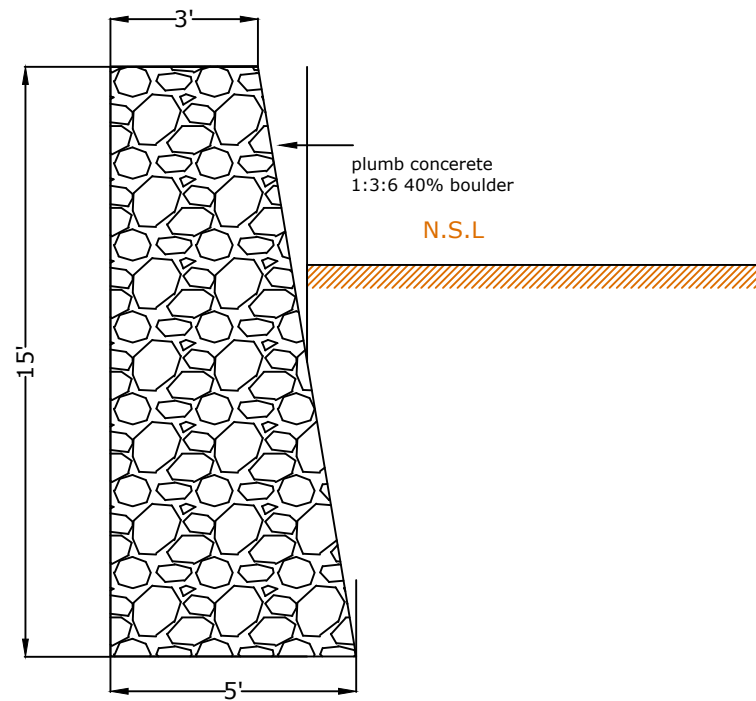
X section plumb concrete
