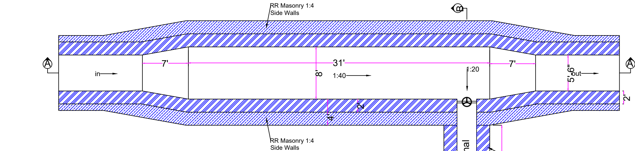
Top View
