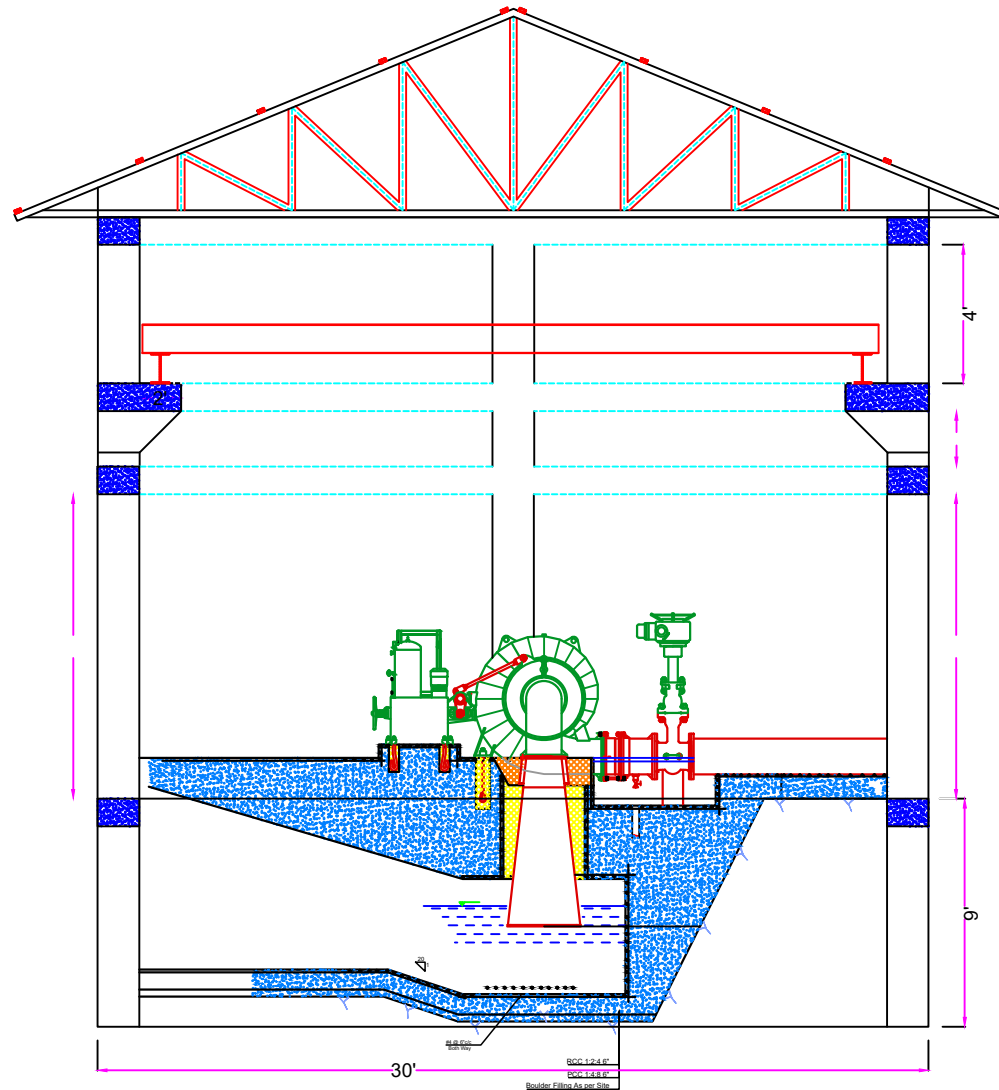
X-SECTION AT B-B
