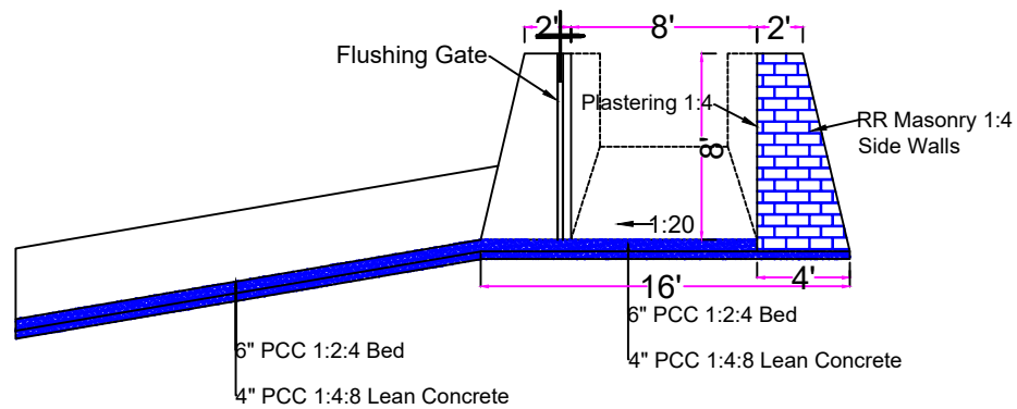
X-Section at B-B
