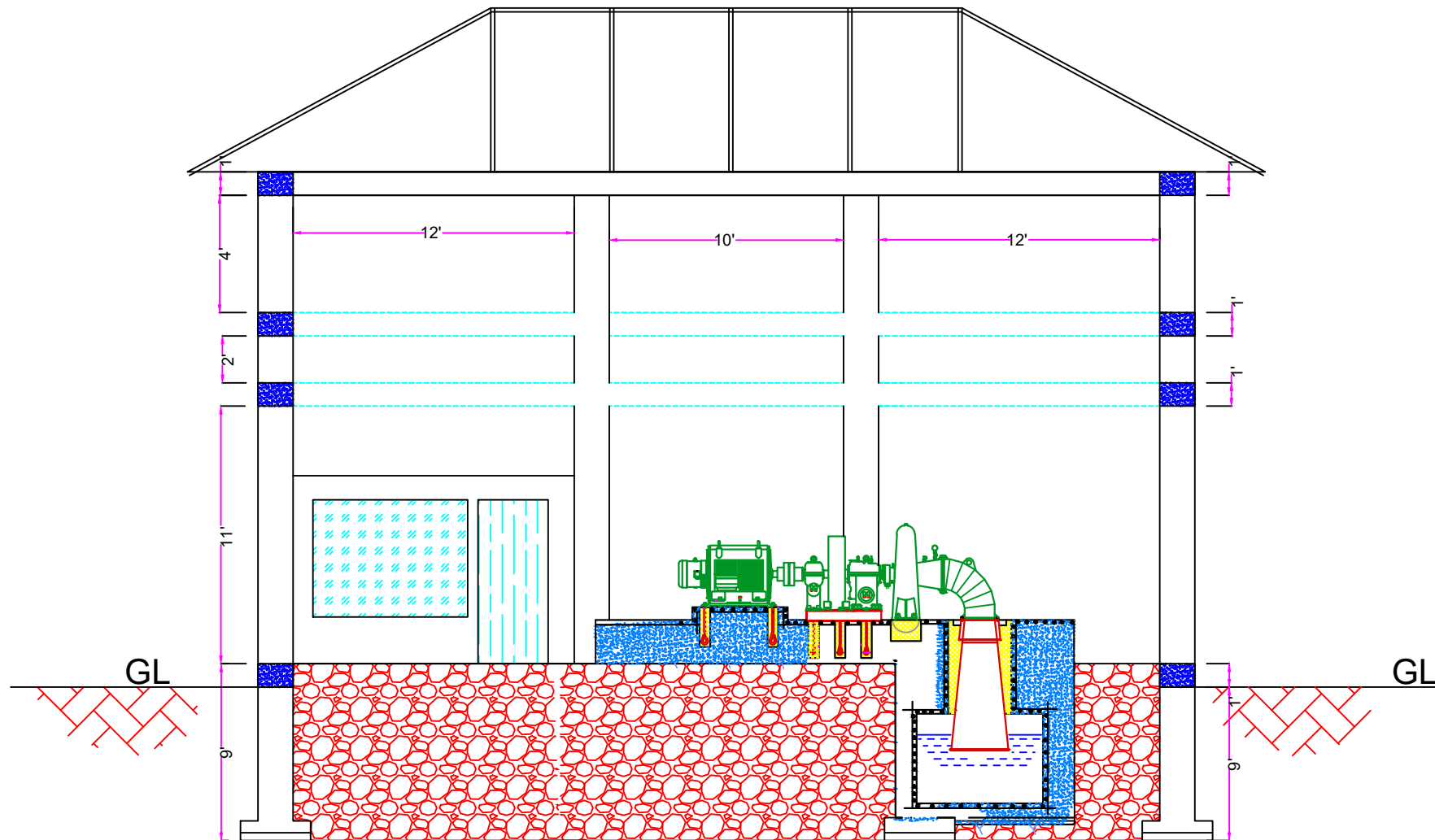
X-SECTION AT A-A
