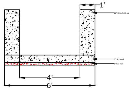
X section of R.C.C
