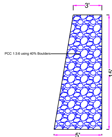
Power House Protection Wall
