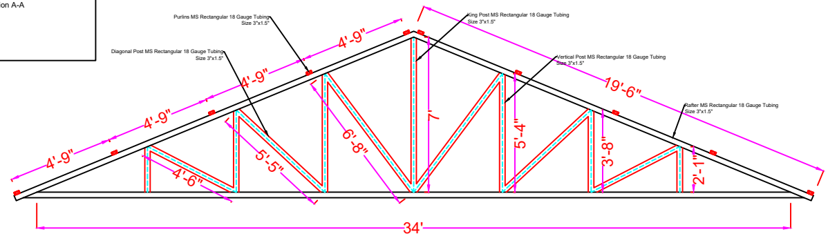
Truss Details
