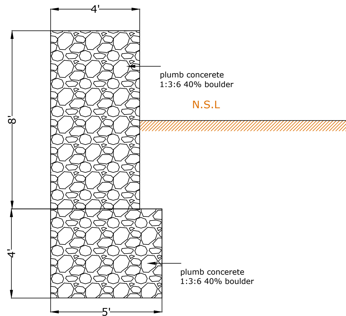
X section plumb concrete
