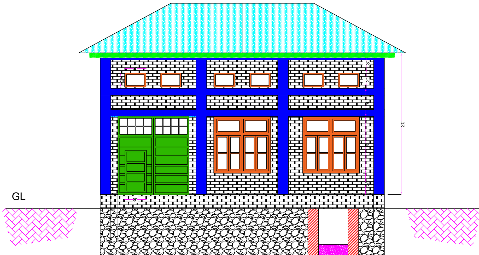
Front Elevation
