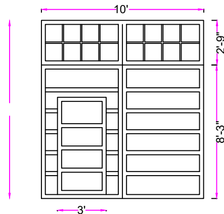
Main Slide Gate
