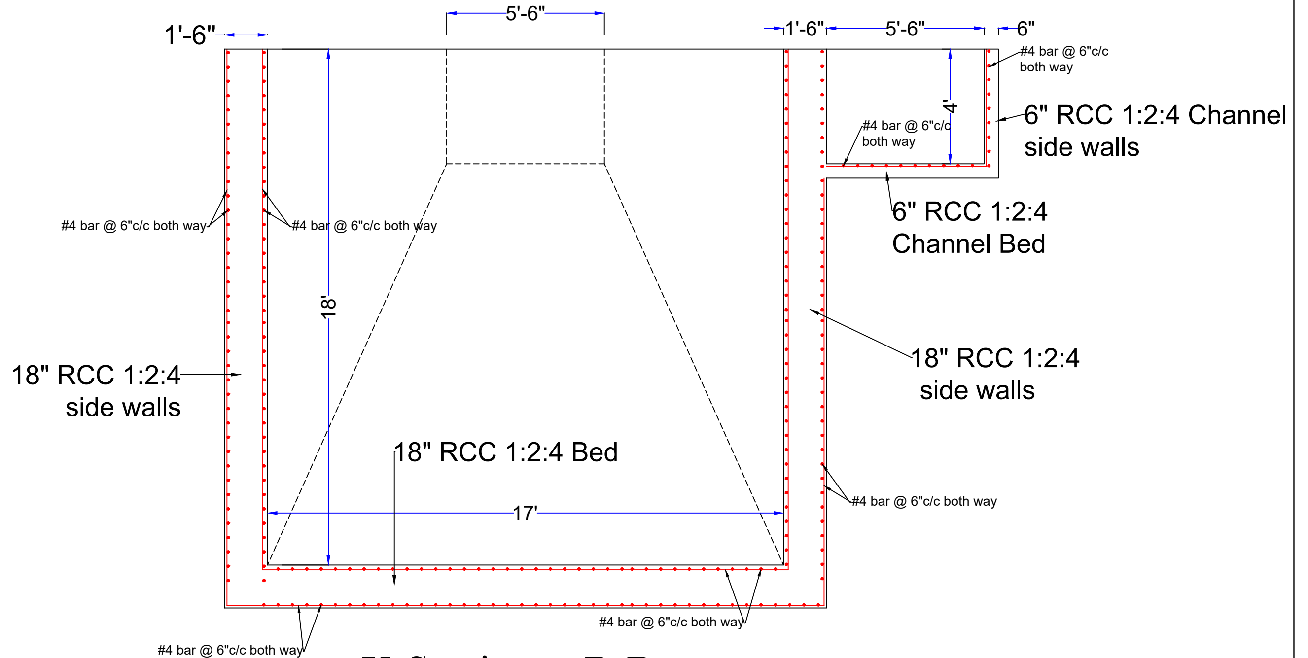
X-Section at B-B
